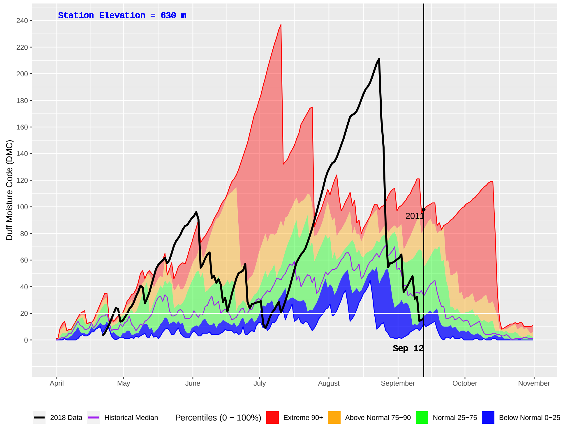
ANDERSON CREEK (977) : Historical (2007–2016) and Current (2018) Daily Duff Moisture Code (DMC)
