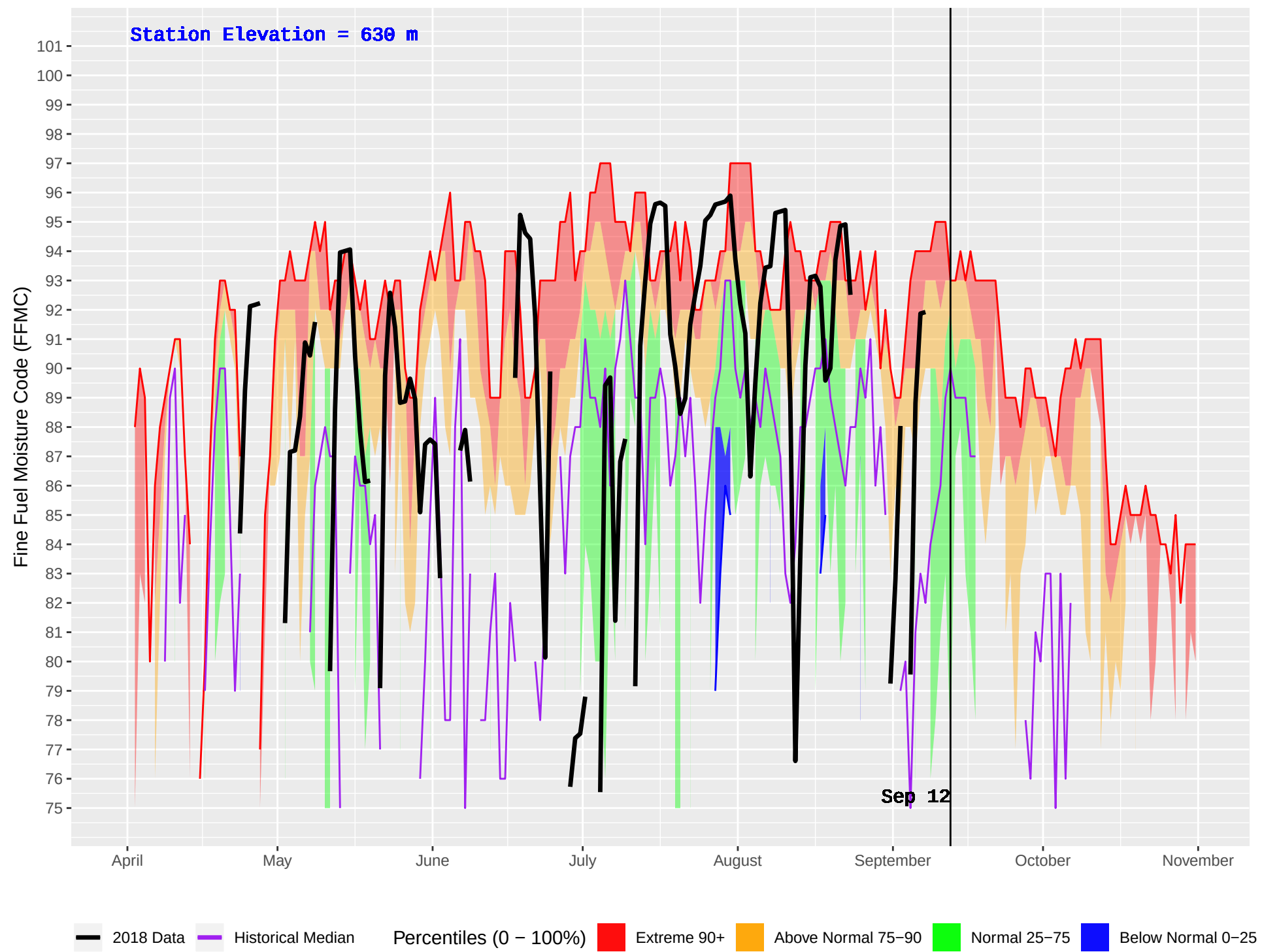
ANDERSON CREEK (977) : Historical (2007–2016) and Current (2018) Daily Fine Fuel Moisture Code (FFMC)
