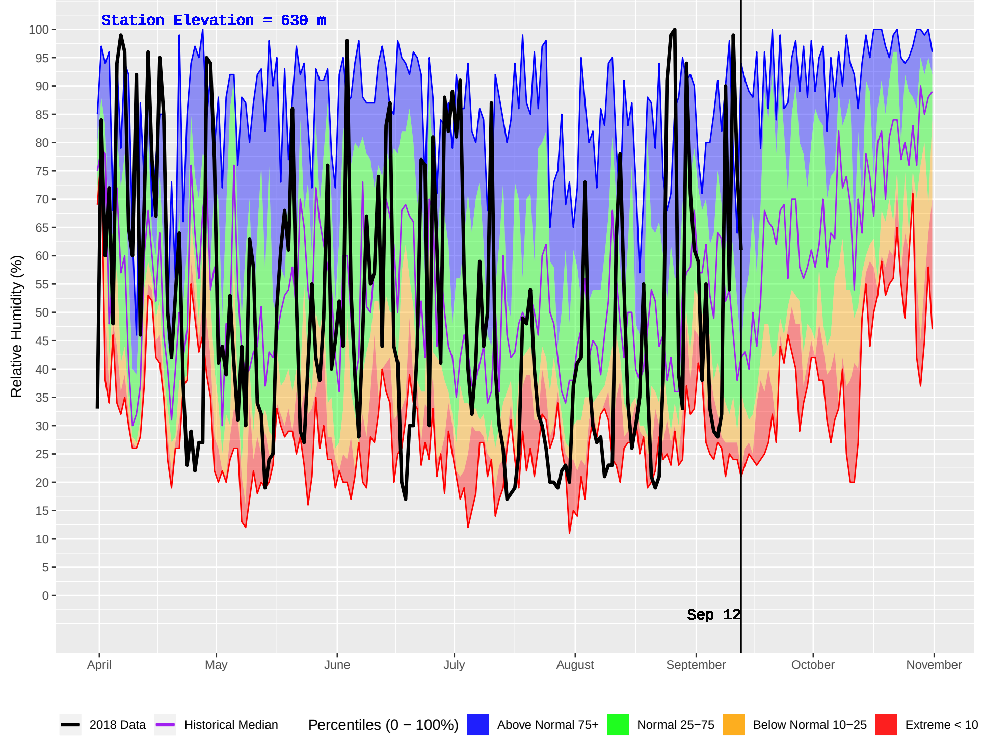
ANDERSON CREEK (977) : Historical (2007–2016) and Current (2018) Daily Relative Humidity
