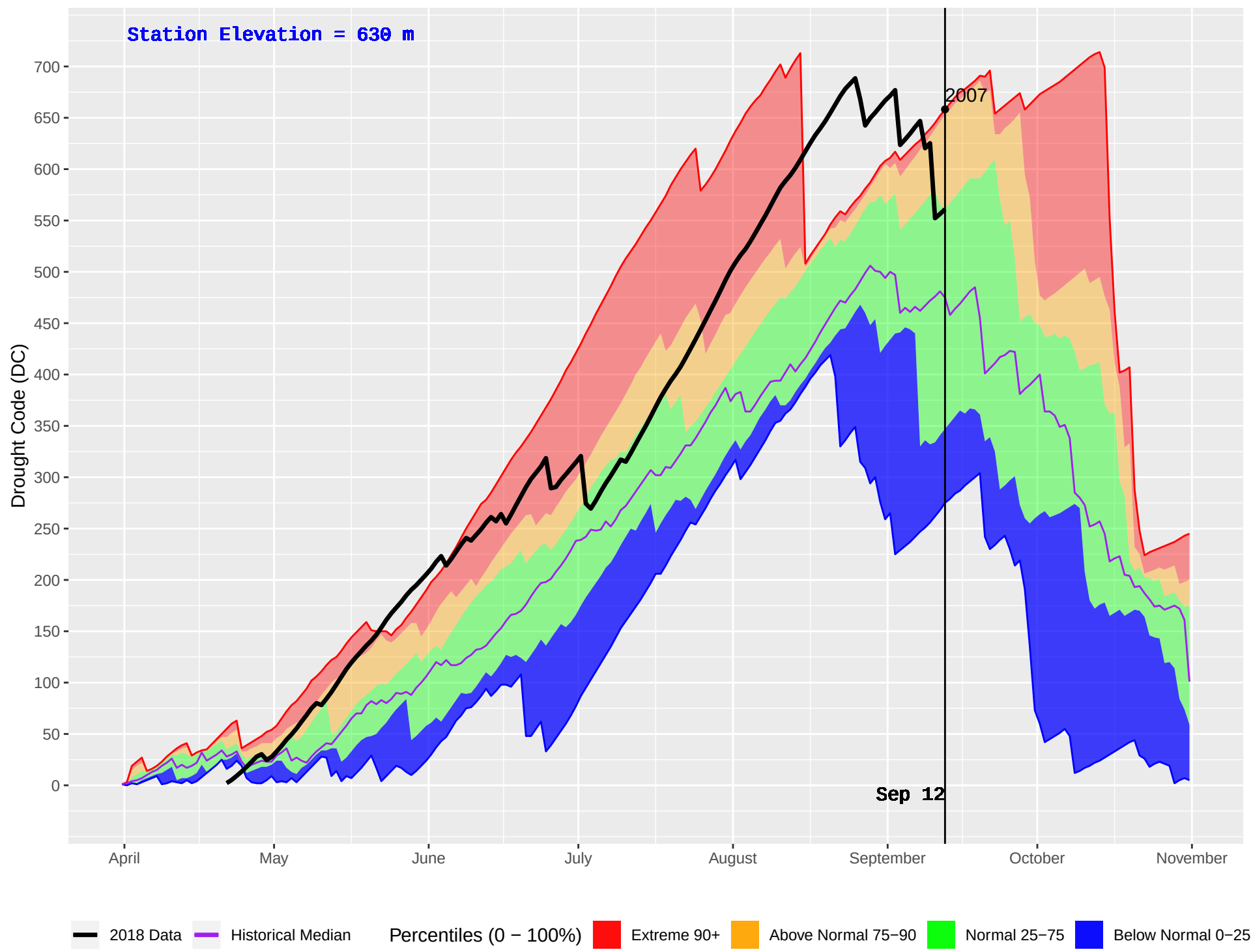
ANDERSON CREEK (977) : Historical (2007–2016) and Current (2018) Daily Drought Code (DC)
