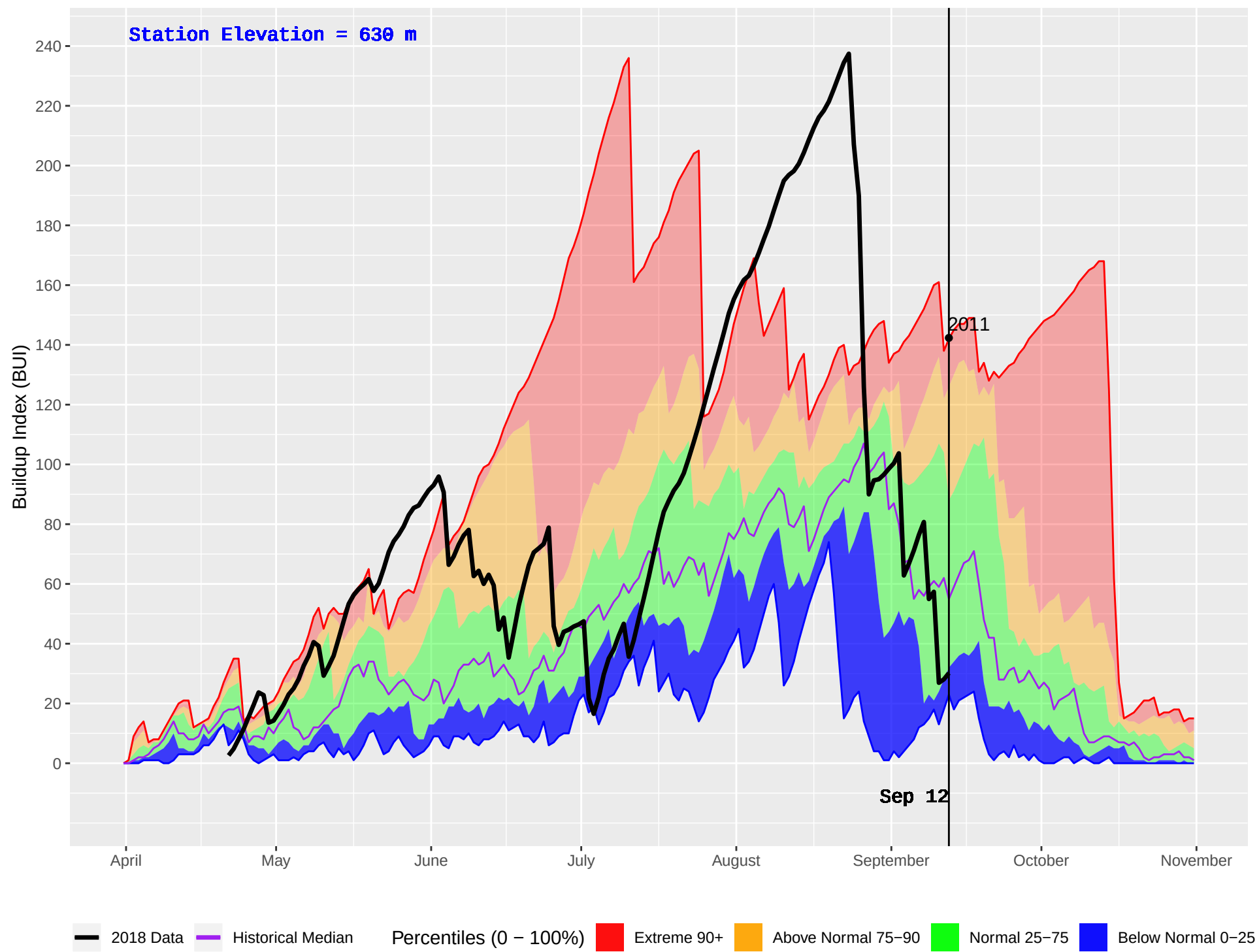
ANDERSON CREEK (977) : Historical (2007–2016) and Current (2018) Daily Buildup Index (BUI)
